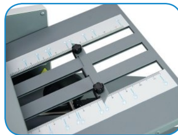
Fold plates are clearly marked for popular folds and are easy to adjust
